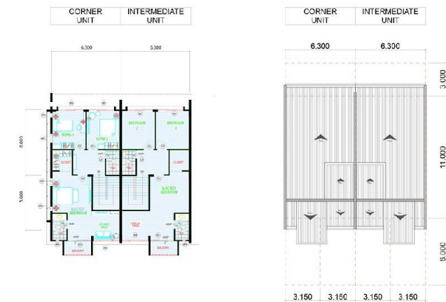
LEVEL 3 FLOOR PLAN SCALE 1:200M
